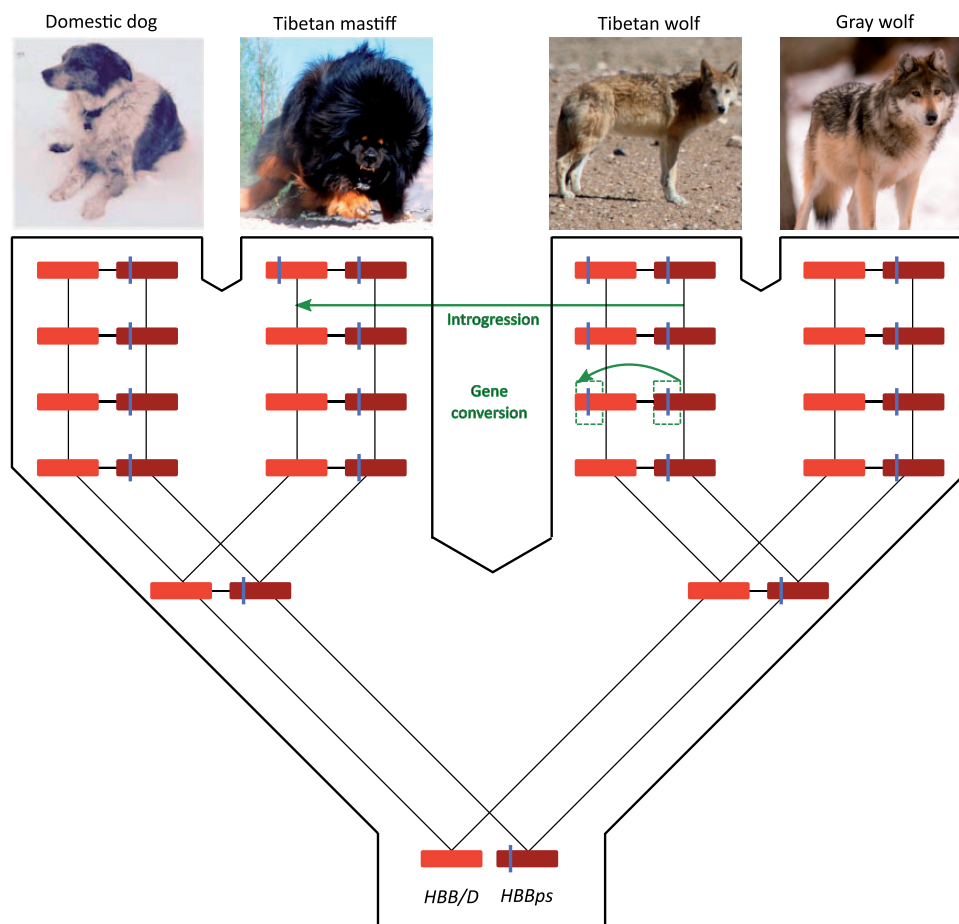
Fig. 2. History of gene conversion between the HBBps pseudogene and the tandemly linked HBB/D gene in Tibetan wolves, and subsequent introgession of the converted HBB/D allele into Tibetan mastiffs. Hash marks denote the paired amino acid replacements, G13S and L14M, which occurred in the dog/wolf ancestor. Image “Tibetan wolf in Changthang” by Stanzin Namgail is licensed under CC BY-SA 4.0 and image “Gray Wolf Standing in the Snow” by Eric Kilby is licensed under CC BY-SA 2.0.
